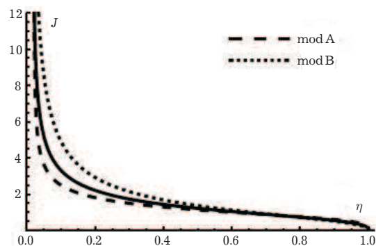
Fig. 5. J -Leverett function.
