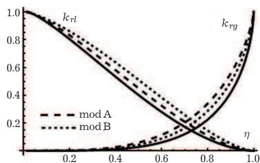
Fig. 6. The relative permeability of liquid k_{rl} and gas k_{rg} phases.
